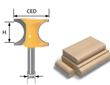
Carbide Tipped Half Round Bit
