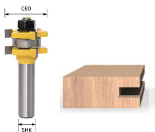
T-joint milling cutter with 3 teeth
