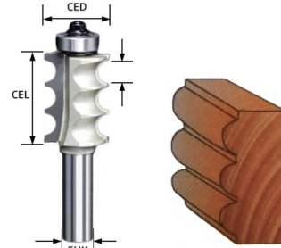
Carbide Tipped Triple Bead Molding Bit
