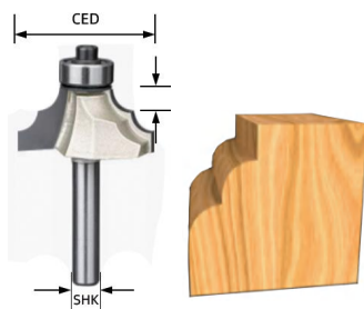
Carbide Tipped Double Roundover Edging Bit
