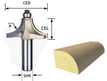
Carbide Tipped Round Over Bit
