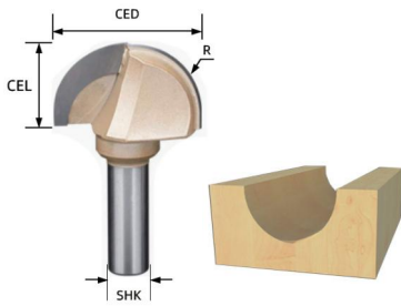
Carbide Tipped Cove Box Bit
