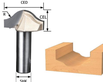
Carbide Tipped Clearing Round Bottom Bit
