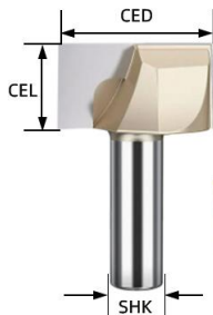
Carbide Tipped Cleaning Bottom Bit
